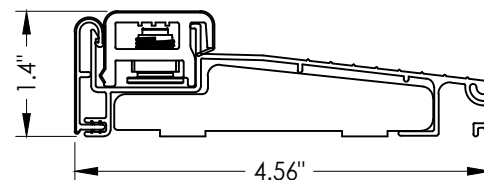
13 INSWING ADJUSTABLE THRESHOLD
