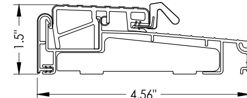
14 OUTSWING THRESHOLD ZOB4565
